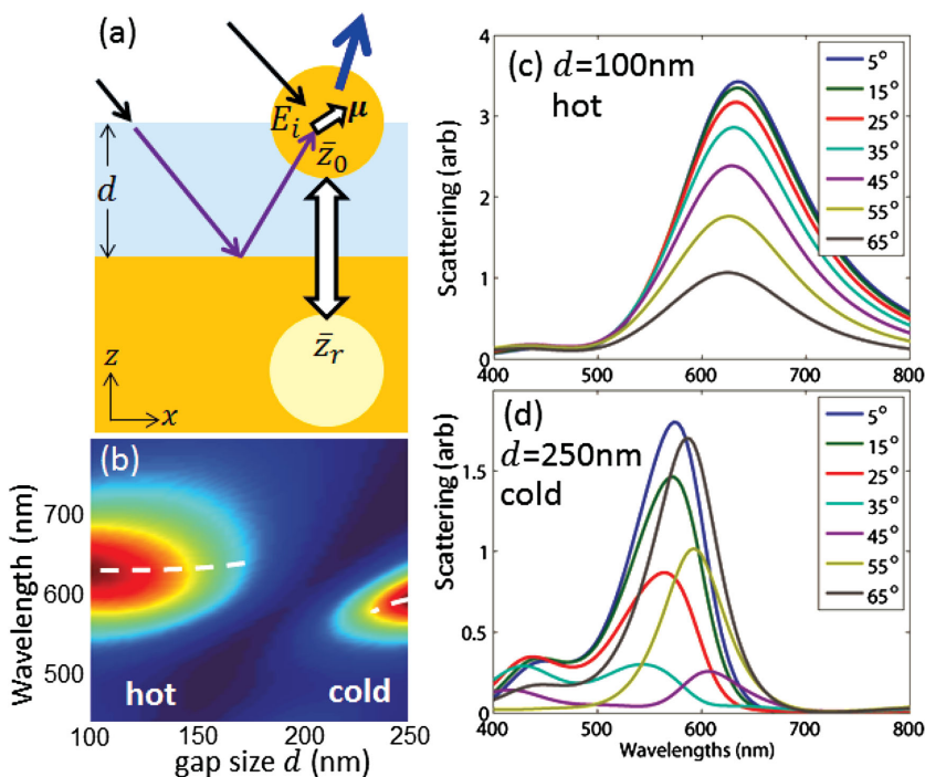
Figure 3. a) Schematic interference paths for scattering Fabry Perot cavity. b) Simulation spectra for 100 nm Au NP on pNIPAM solvated film, as it collapses from 250 to 100 nm when heated to 35 °C. Simulated scattering of Au NPoM with pNIPAM spacer thickness of c) 100 nm and d) 250 nm at different incident angles.
